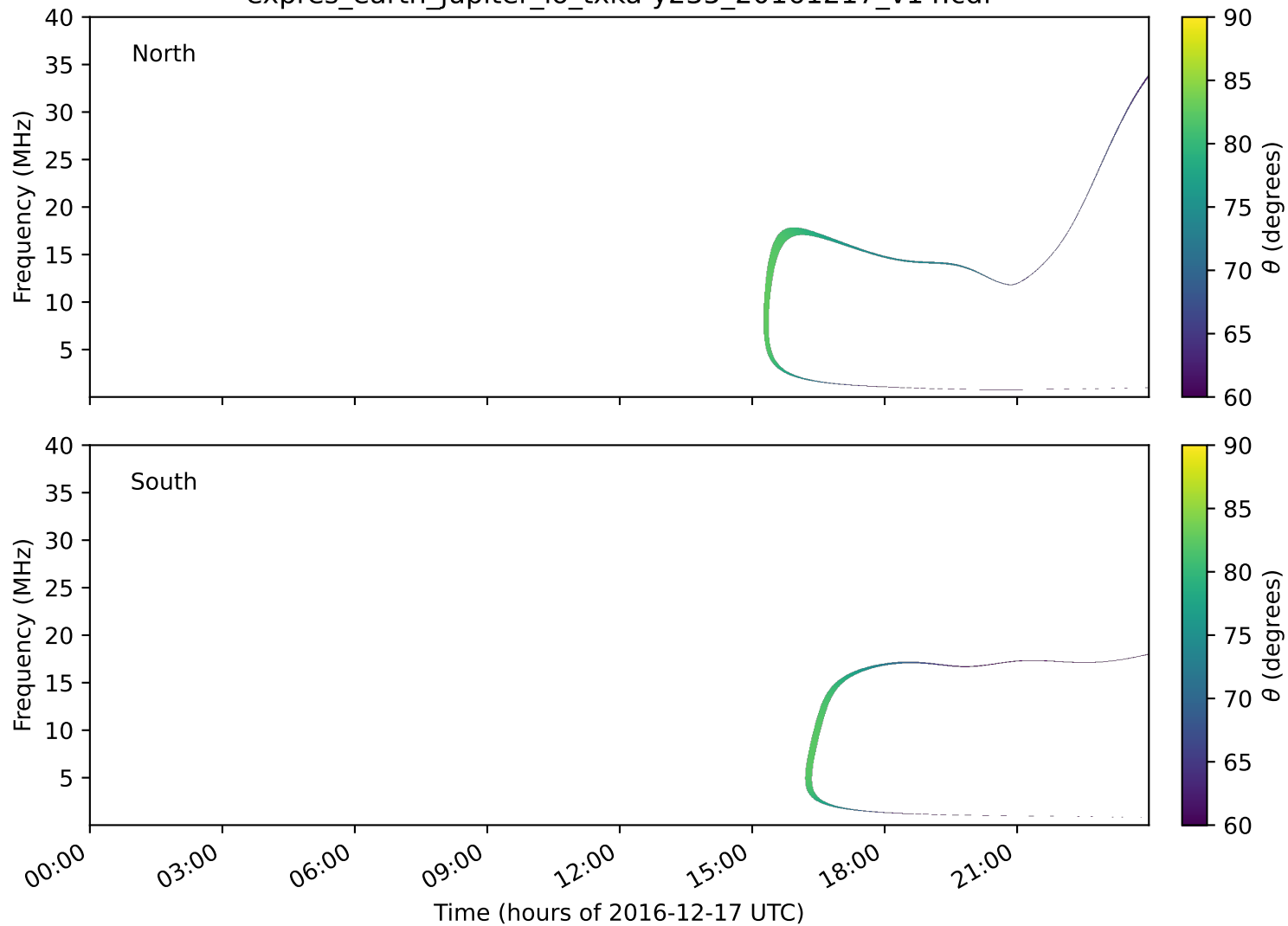
expres_earth_jupiter_io_txka-y235_20161217_v14.cdf
