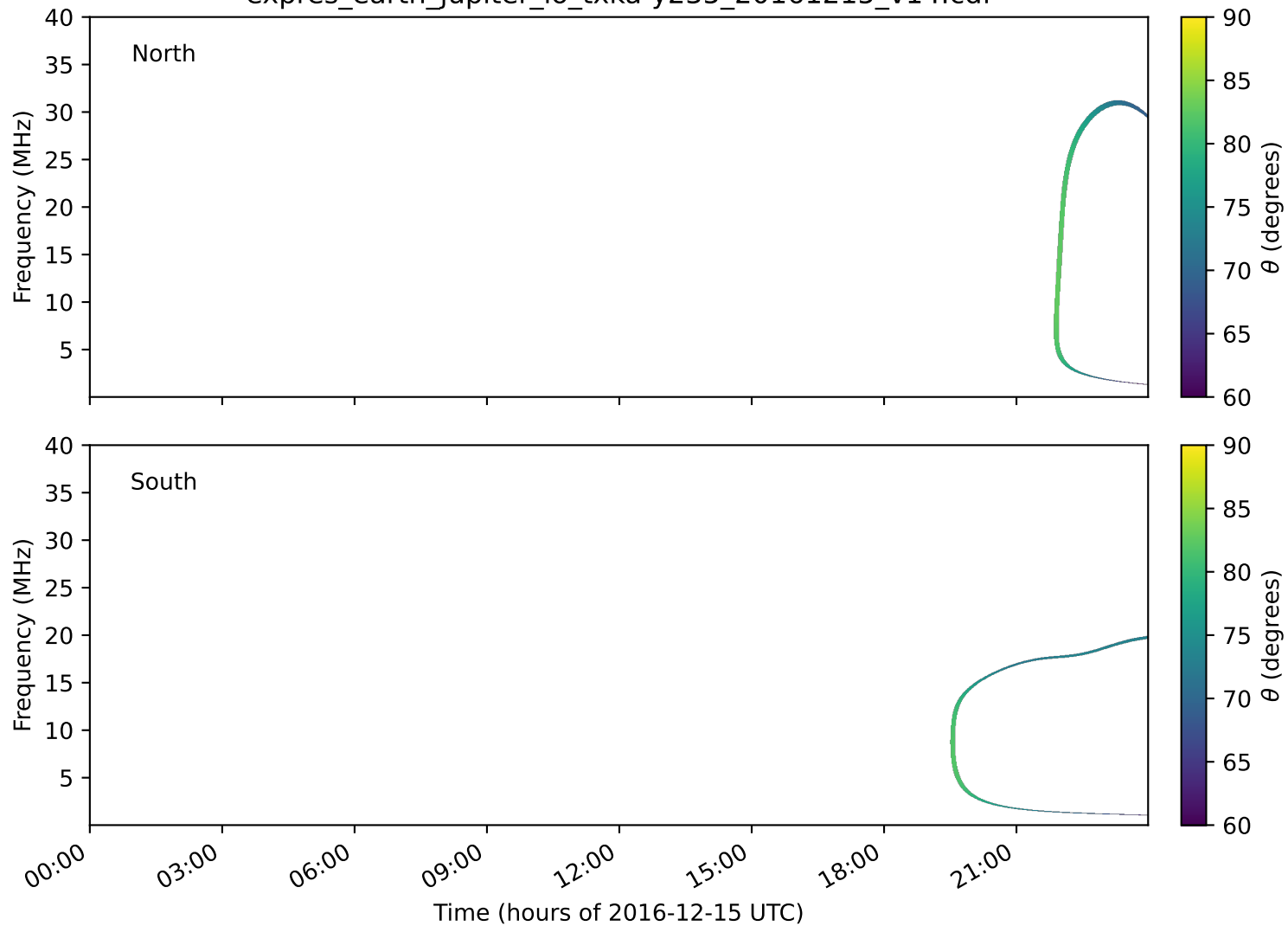
expres_earth_jupiter_io_txka-y235_20161215_v14.cdf
