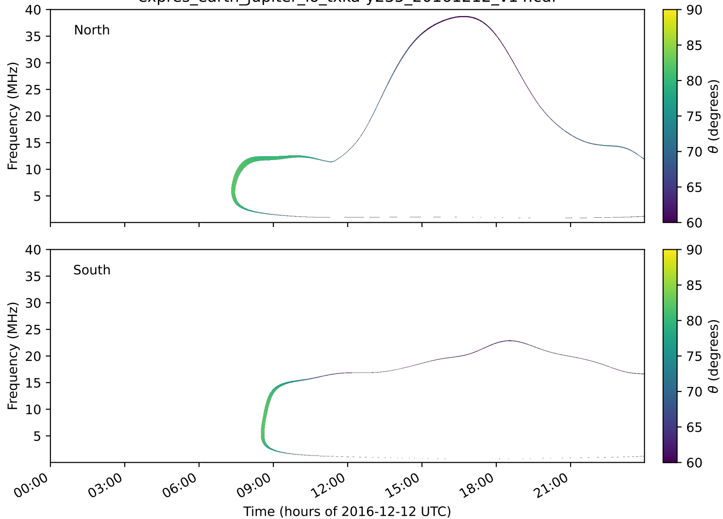
expres_earth_jupiter_io_txka-y235_20161212_v14.cdf
