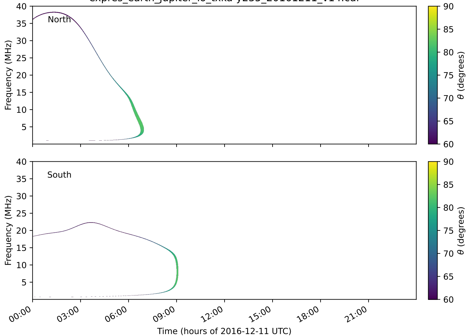
expres_earth_jupiter_io_txka-y235_20161211_v14.cdf
