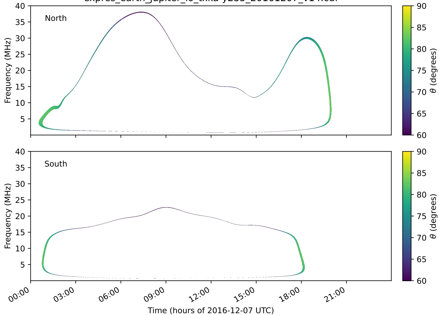
expres_earth_jupiter_io_txka-y235_20161207_v14.cdf
