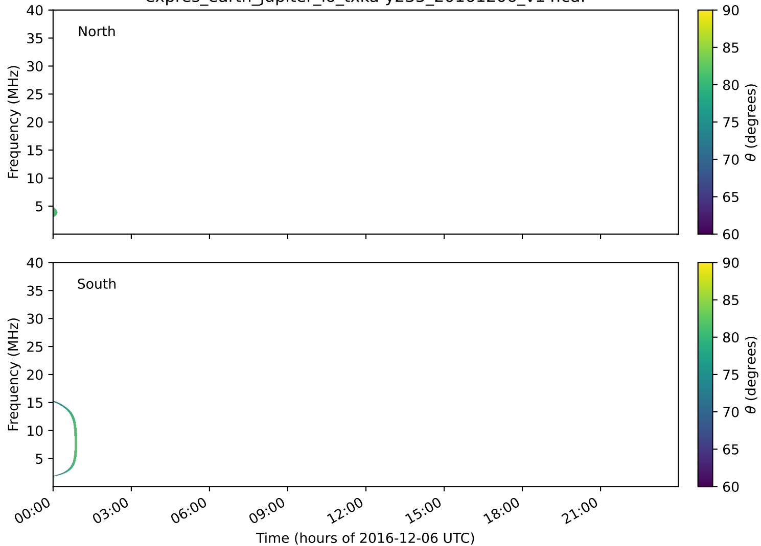
expres_earth_jupiter_io_txka-y235_20161206_v14.cdf
