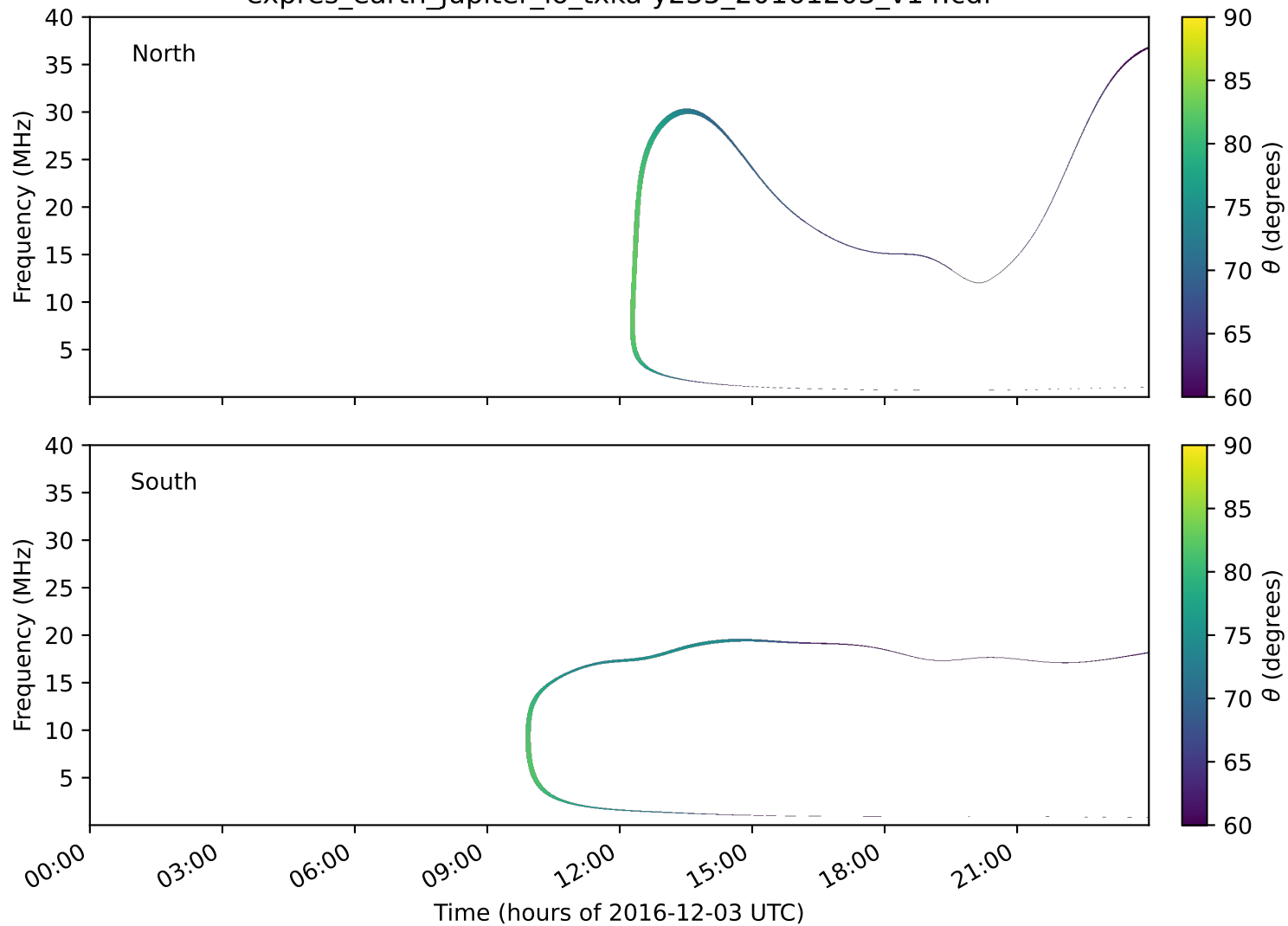
expres_earth_jupiter_io_txka-y235_20161203_v14.cdf
