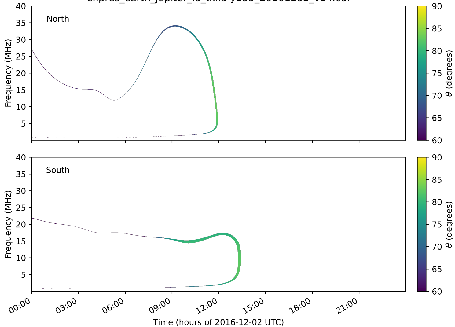
expres_earth_jupiter_io_txka-y235_20161202_v14.cdf
