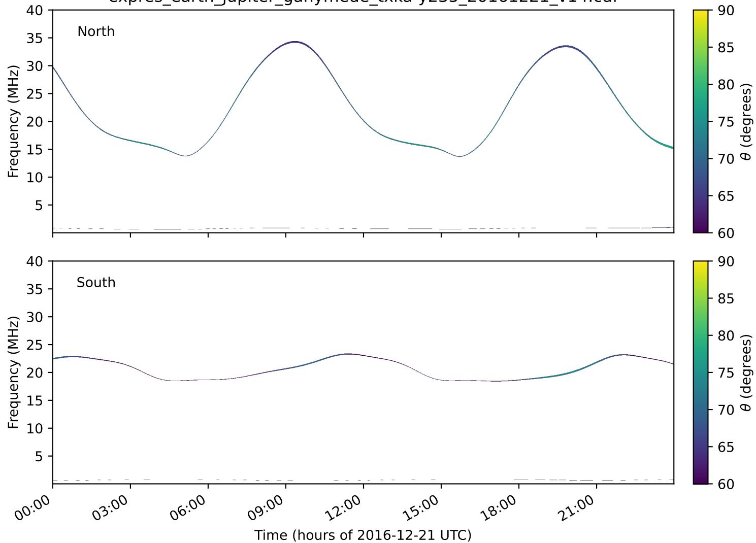
expres_earth_jupiter_ganymede_txka-y235_20161221_v14.cdf
