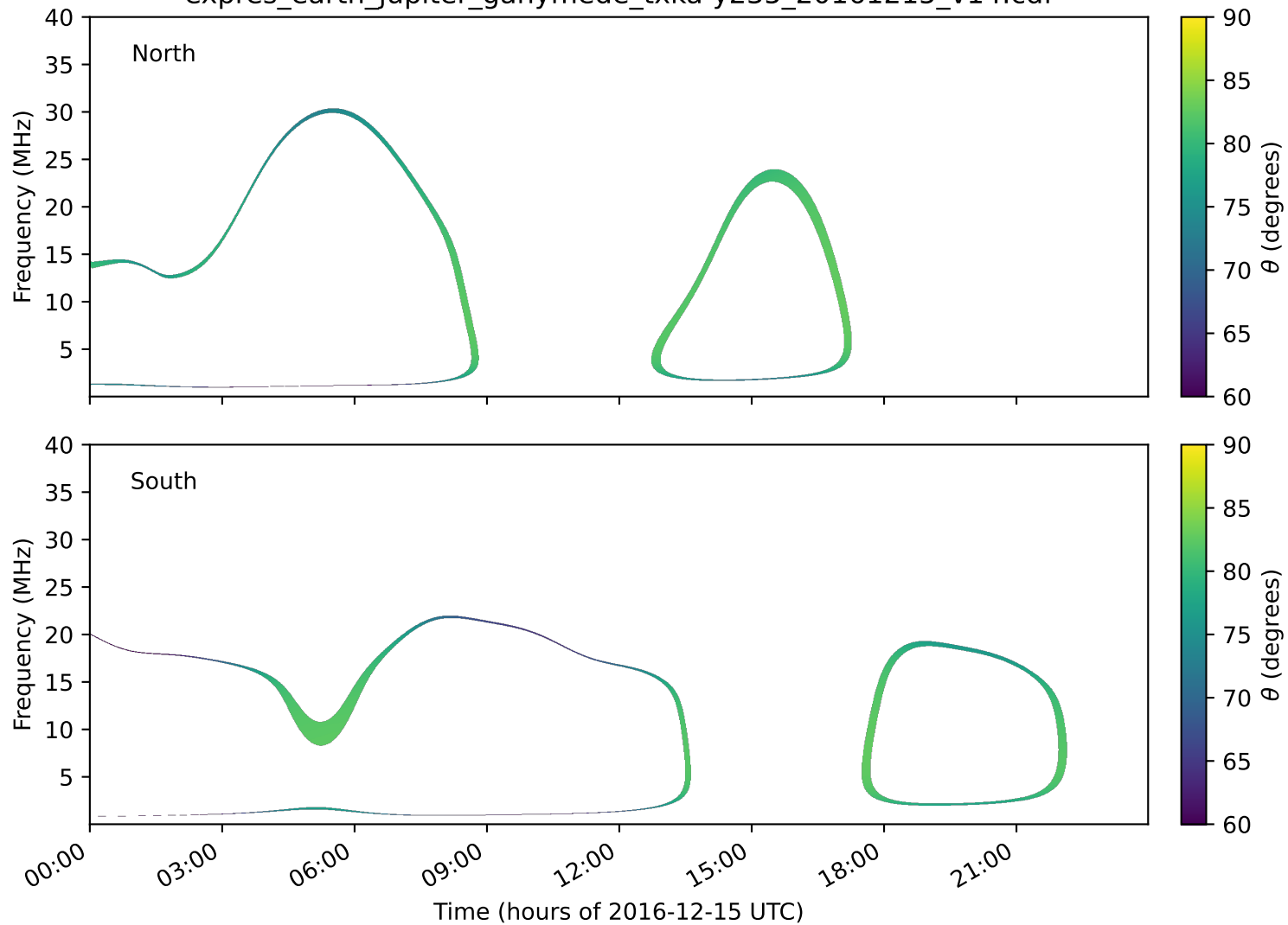
expres_earth_jupiter_ganymede_txka-y235_20161215_v14.cdf
