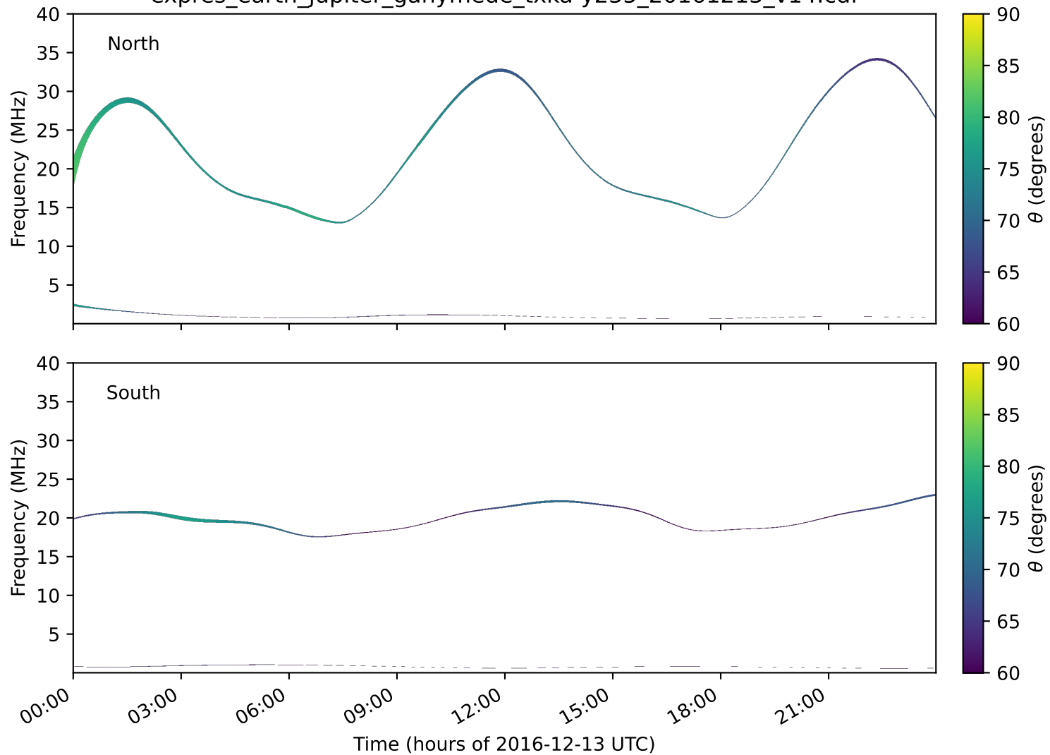
expres_earth_jupiter_ganymede_txka-y235_20161213_v14.cdf
