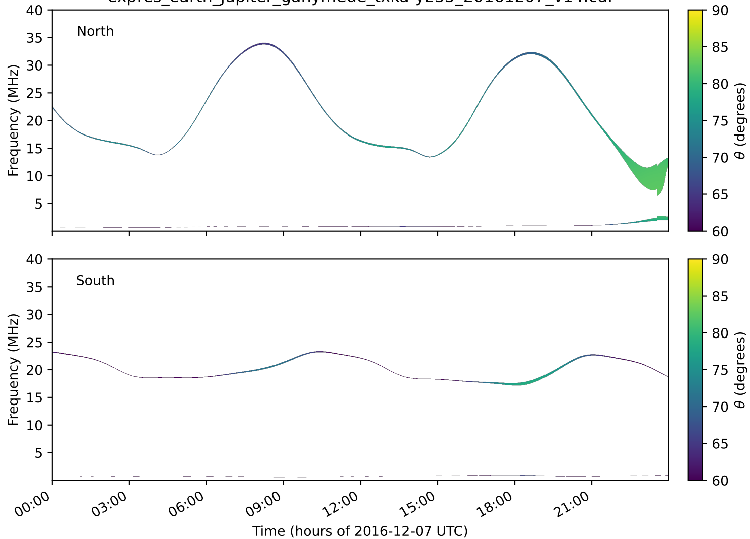
expres_earth_jupiter_ganymede_txka-y235_20161207_v14.cdf
