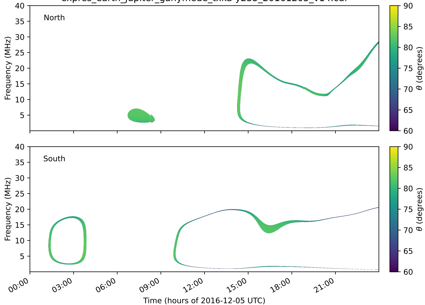
expres_earth_jupiter_ganymede_txka-y235_20161205_v14.cdf
