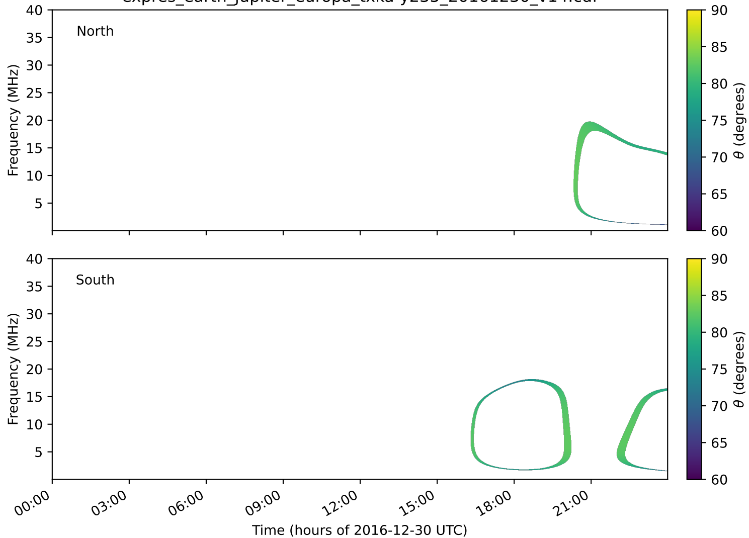
expres_earth_jupiter_europa_txka-y235_20161230_v14.cdf
