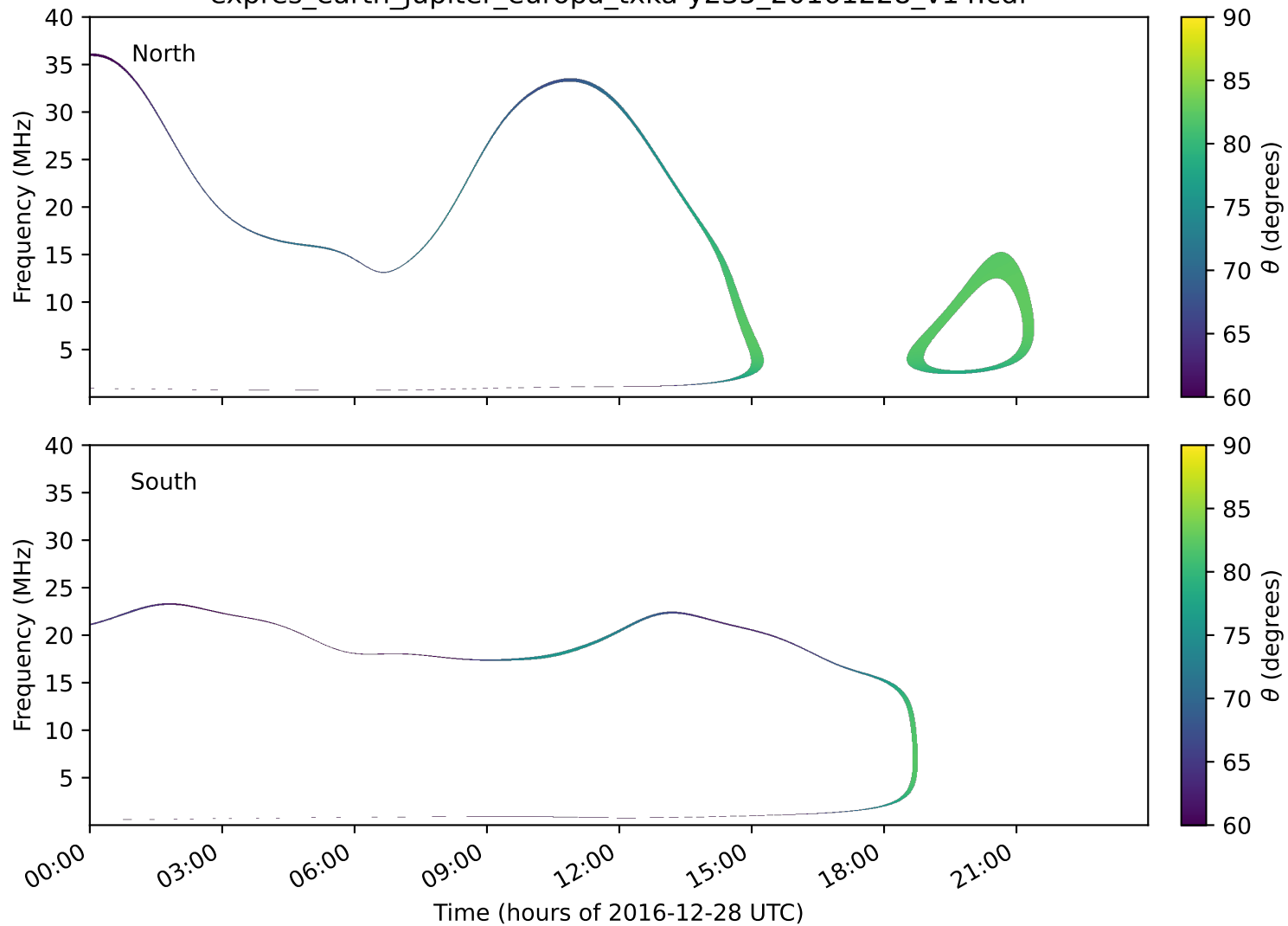
expres_earth_jupiter_europa_txka-y235_20161228_v14.cdf
