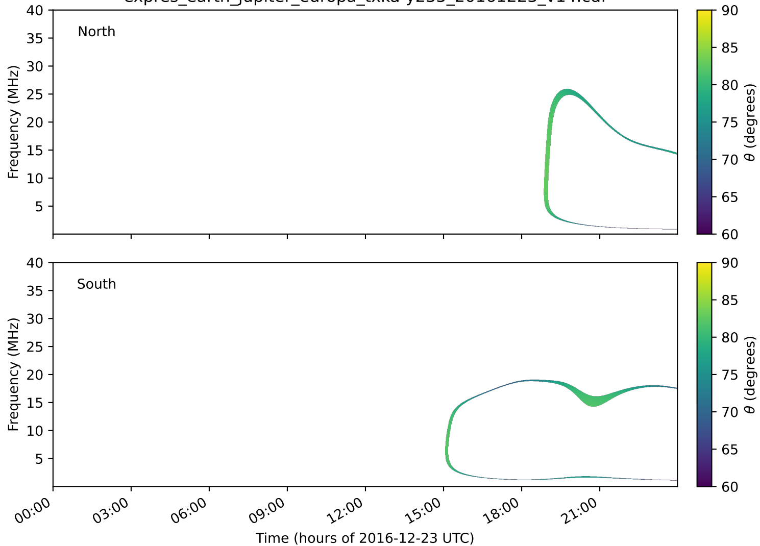
expres_earth_jupiter_europa_txka-y235_20161223_v14.cdf
