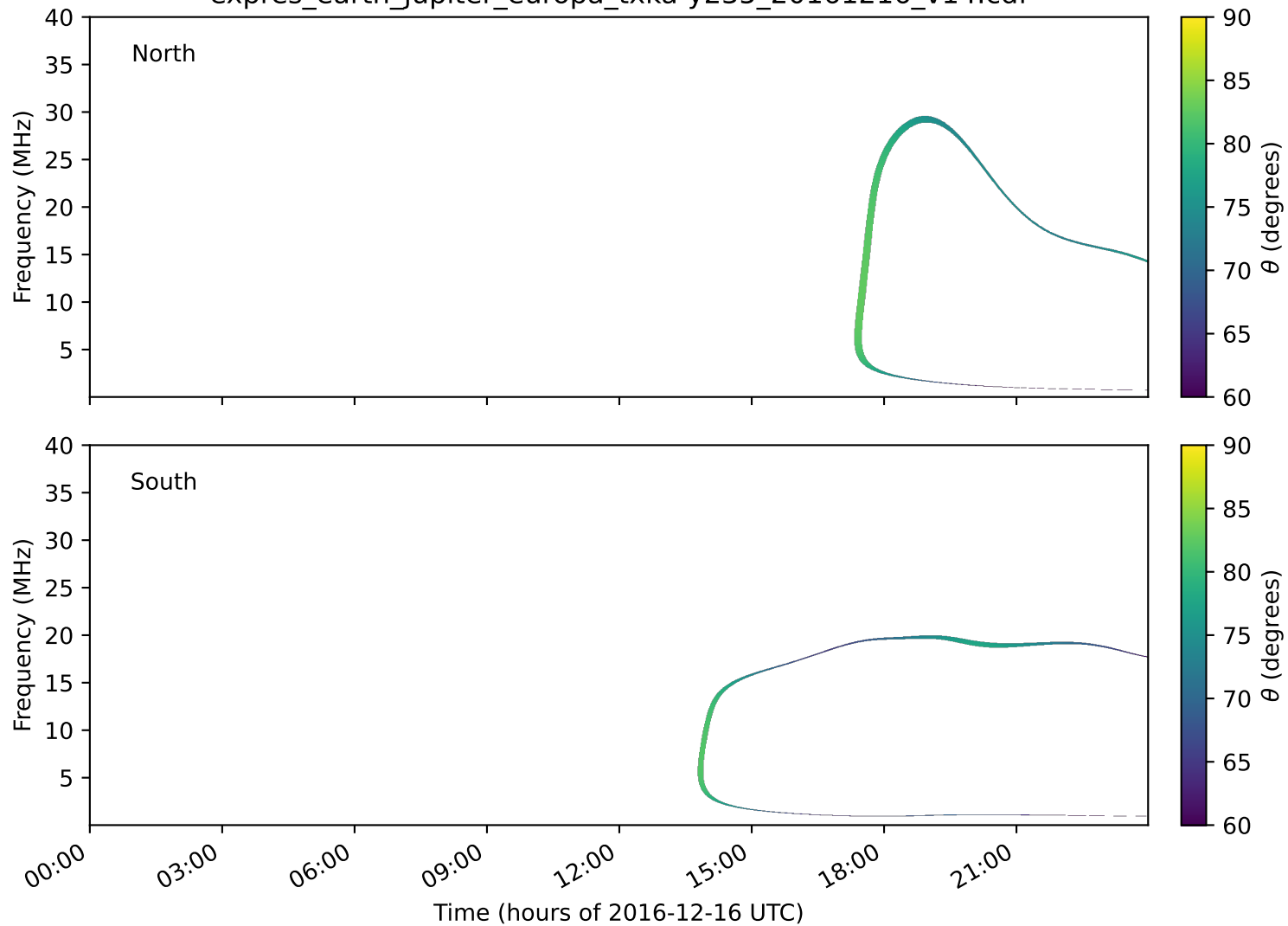
expres_earth_jupiter_europa_txka-y235_20161216_v14.cdf
