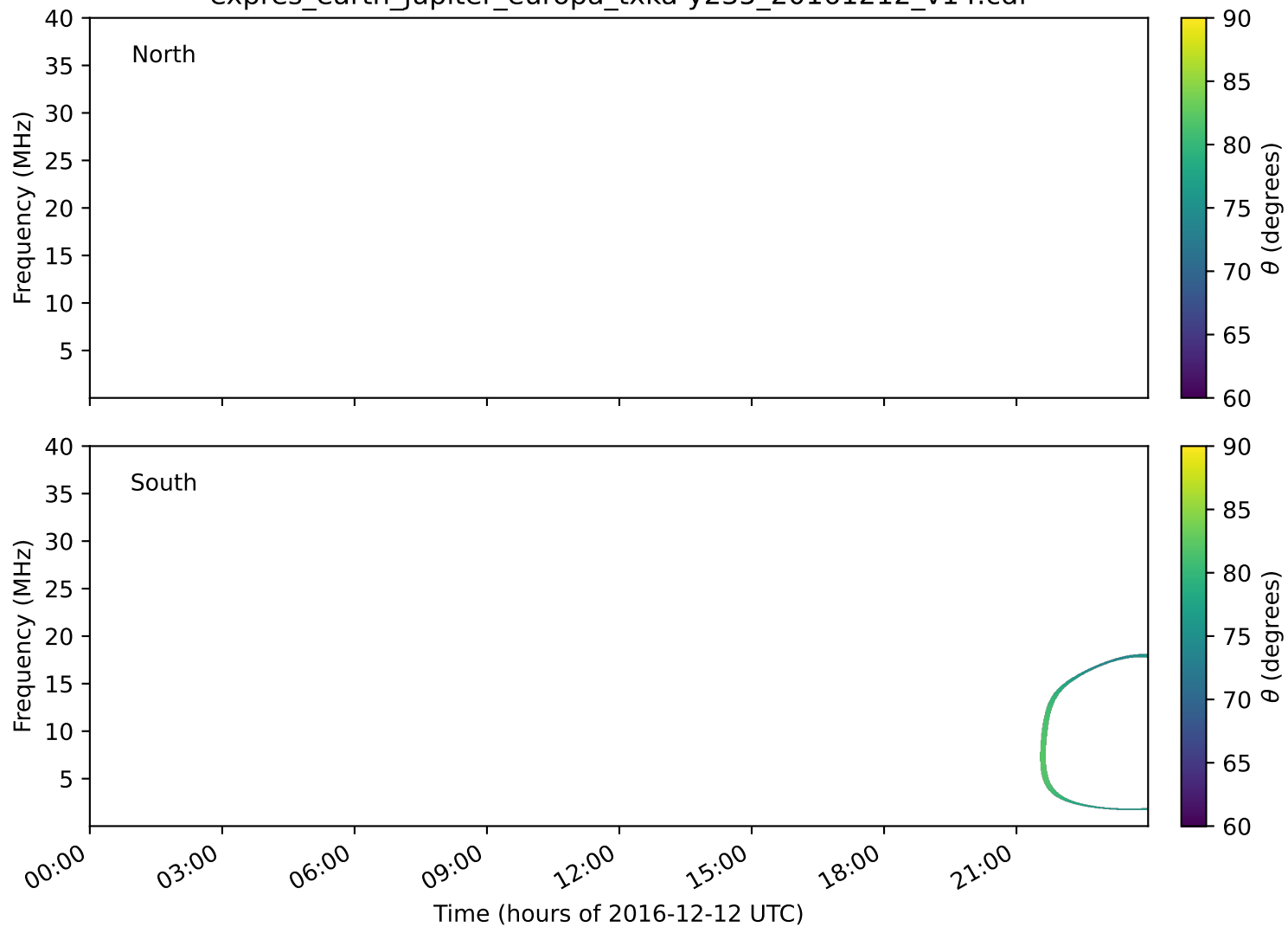
expres_earth_jupiter_europa_txka-y235_20161212_v14.cdf
