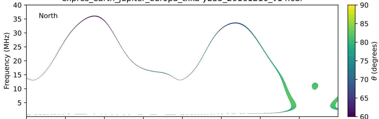
expres_earth_jupiter_europa_txka-y235_20161210_v14.cdf
