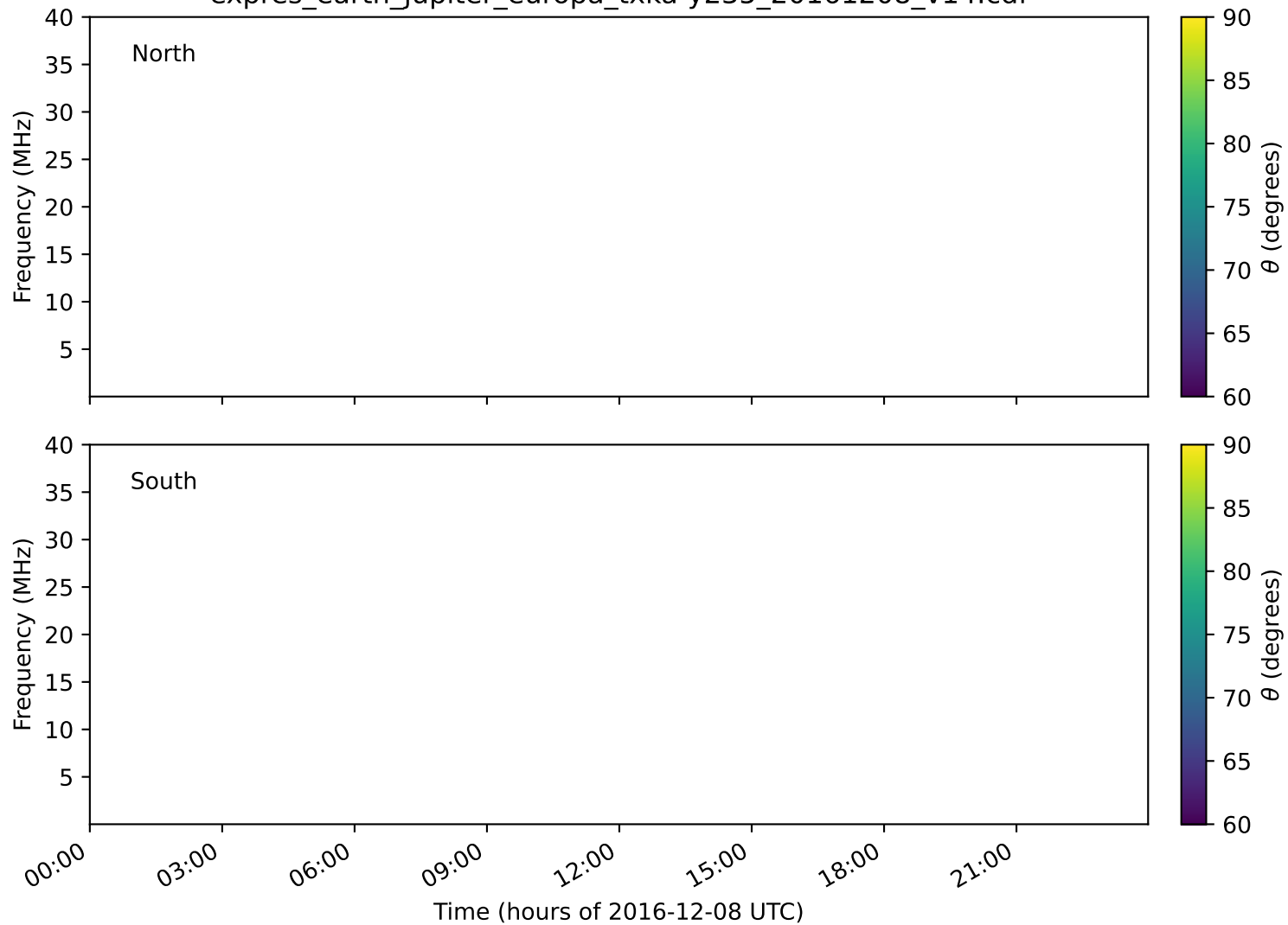
expres_earth_jupiter_europa_txka-y235_20161208_v14.cdf
