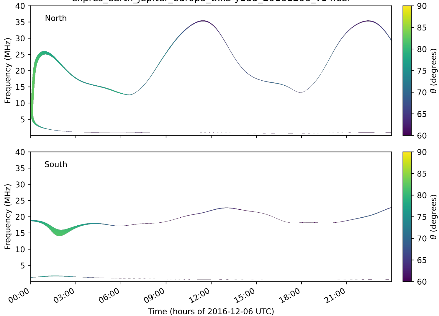
expres_earth_jupiter_europa_txka-y235_20161206_v14.cdf
