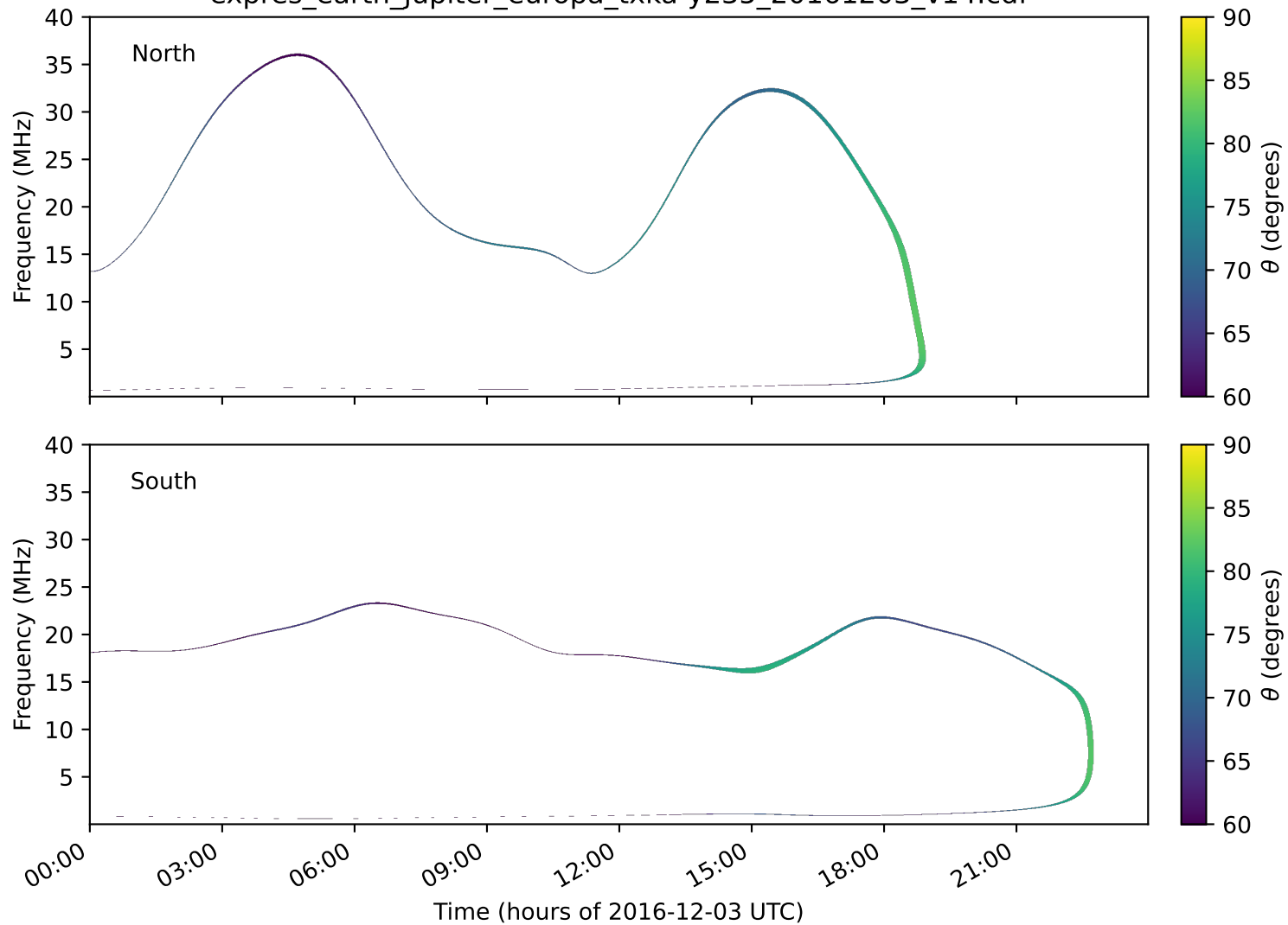
expres_earth_jupiter_europa_txka-y235_20161203_v14.cdf
