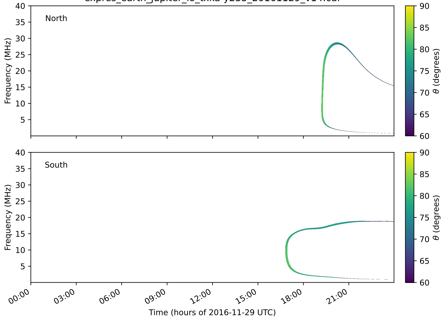
expres_earth_jupiter_io_txka-y235_20161129_v14.cdf
