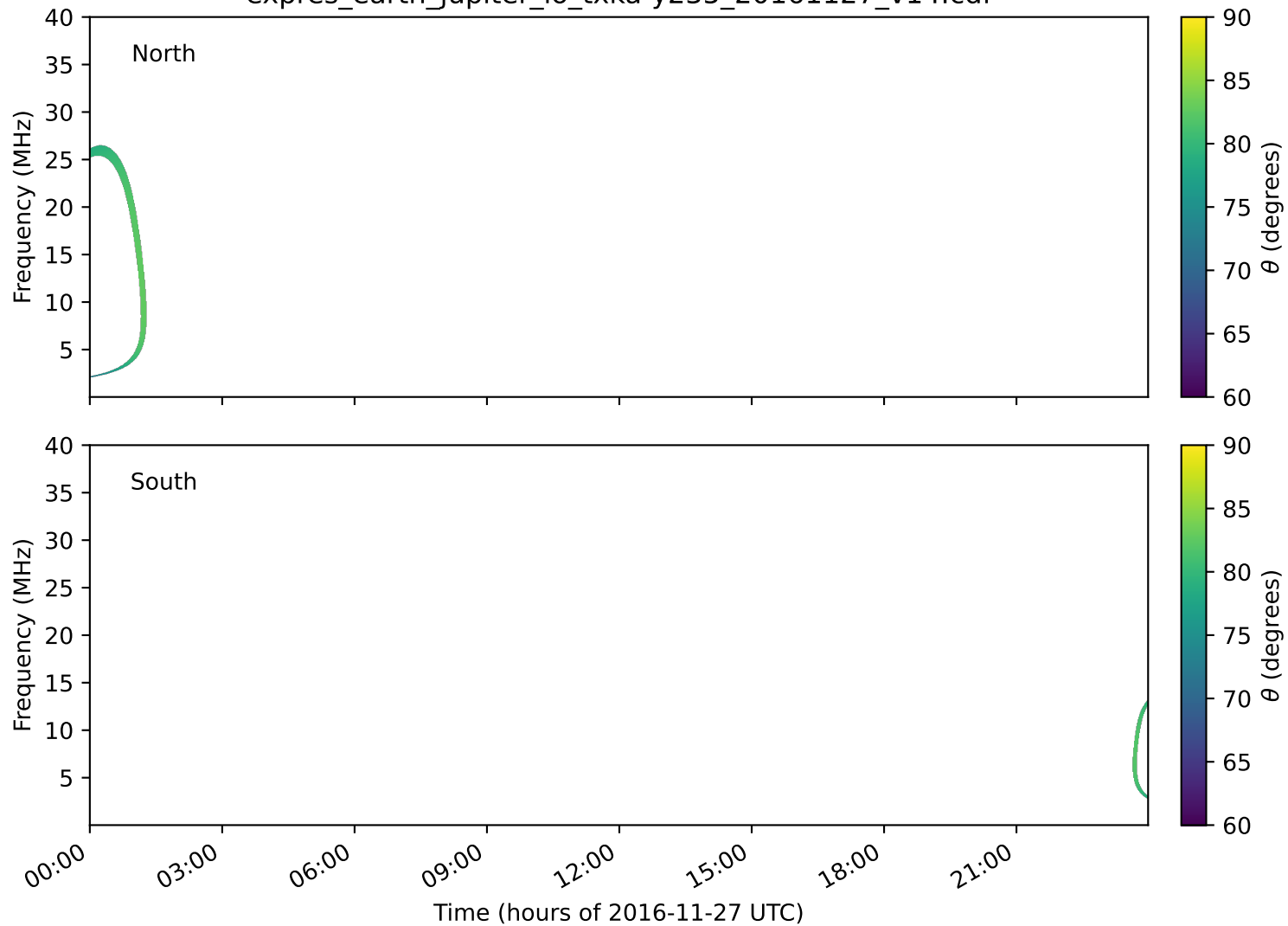
expres_earth_jupiter_io_txka-y235_20161127_v14.cdf
