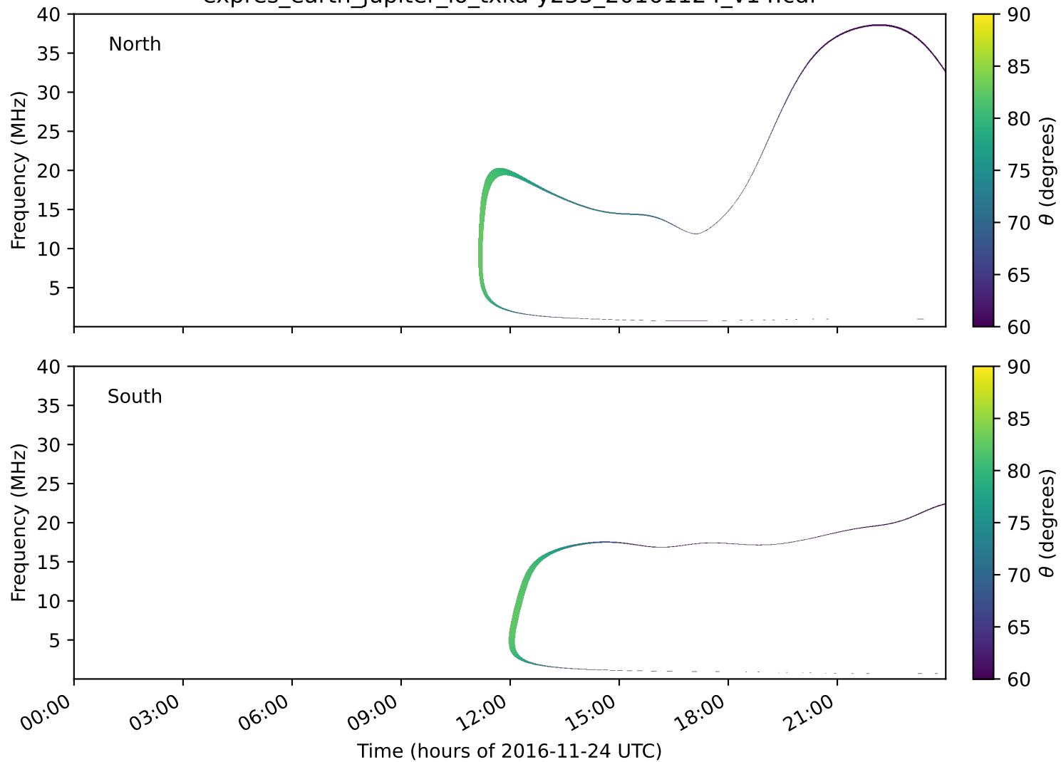
expres_earth_jupiter_io_txka-y235_20161124_v14.cdf
