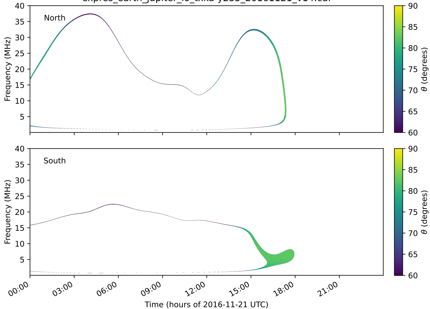
expres_earth_jupiter_io_txka-y235_20161121_v14.cdf
