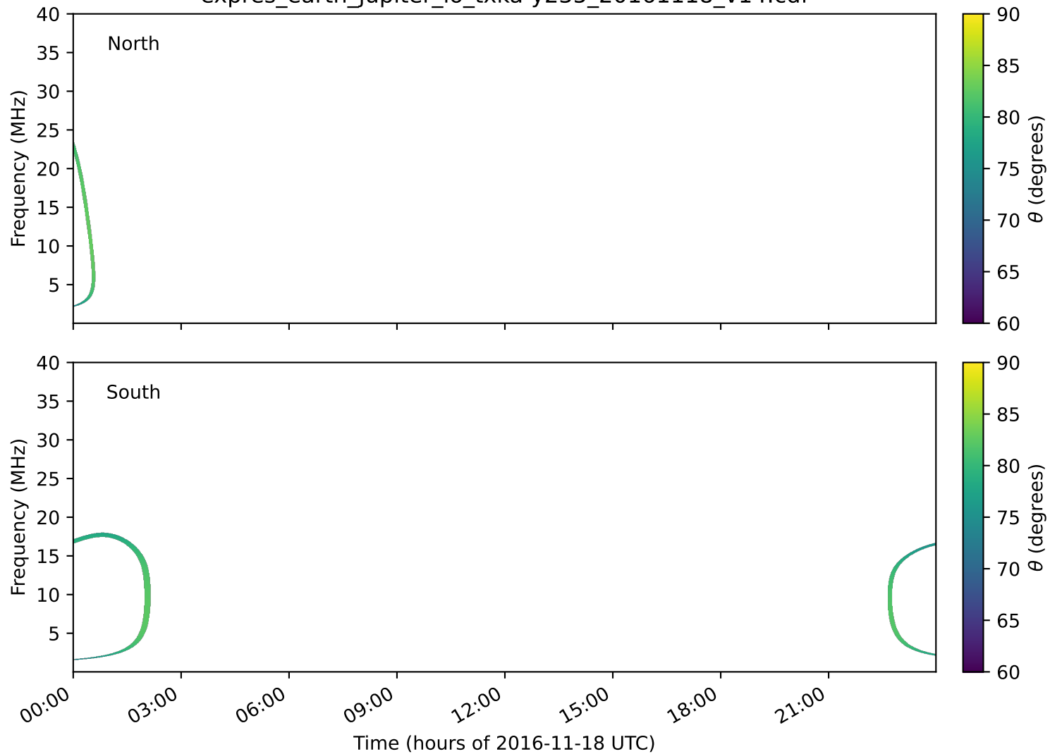
expres_earth_jupiter_io_txka-y235_20161118_v14.cdf
