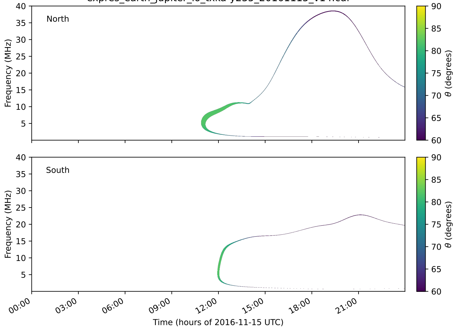
expres_earth_jupiter_io_txka-y235_20161115_v14.cdf
