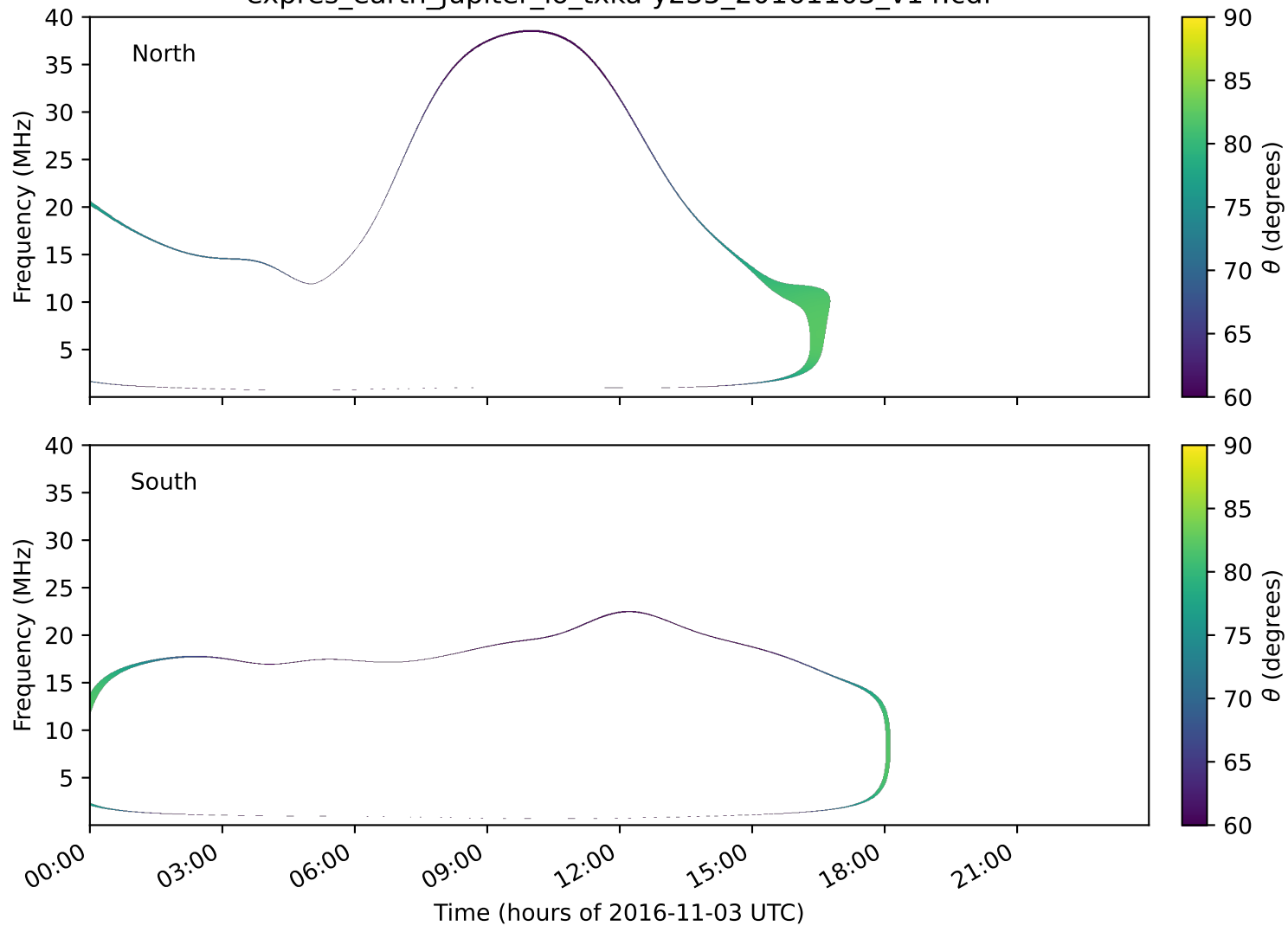
expres_earth_jupiter_io_txka-y235_20161103_v14.cdf
