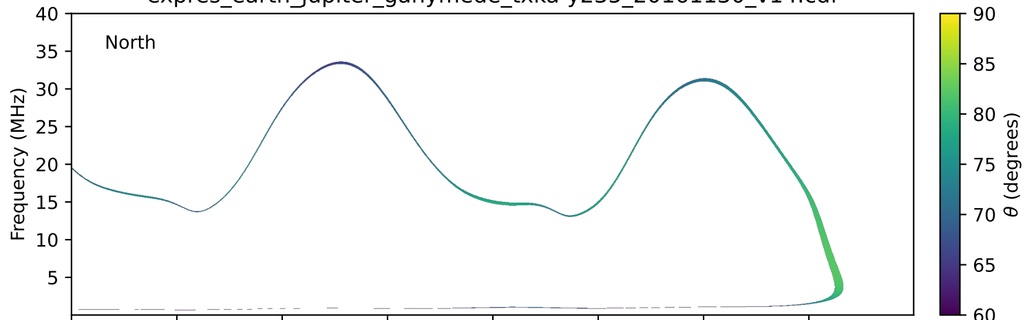
expres_earth_jupiter_ganymede_txka-y235_20161130_v14.cdf
