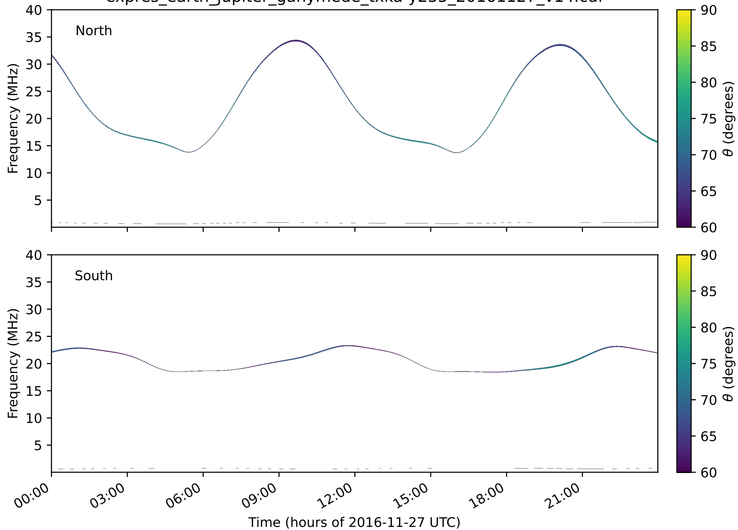
expres_earth_jupiter_ganymede_txka-y235_20161127_v14.cdf
