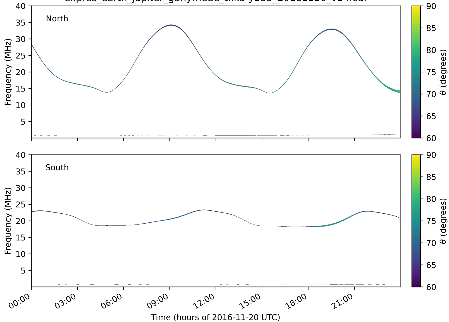
expres_earth_jupiter_ganymede_txka-y235_20161120_v14.cdf
