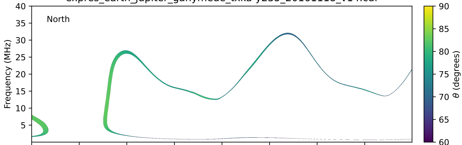
expres_earth_jupiter_ganymede_txka-y235_20161118_v14.cdf
