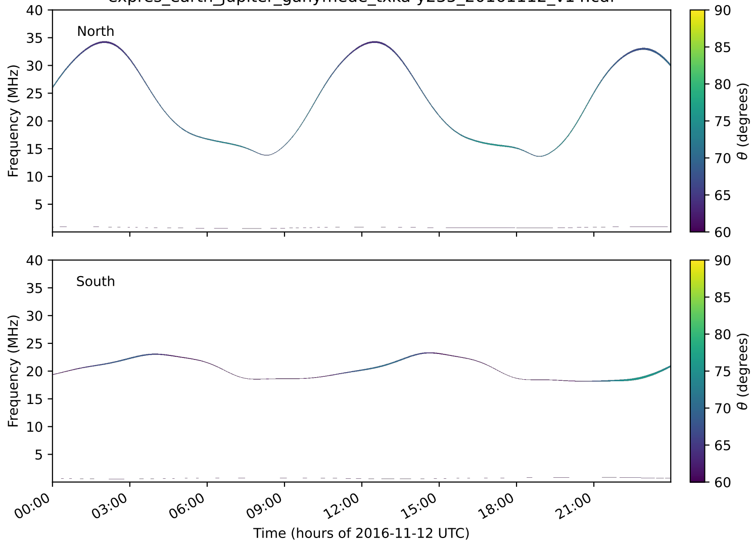
expres_earth_jupiter_ganymede_txka-y235_20161112_v14.cdf
