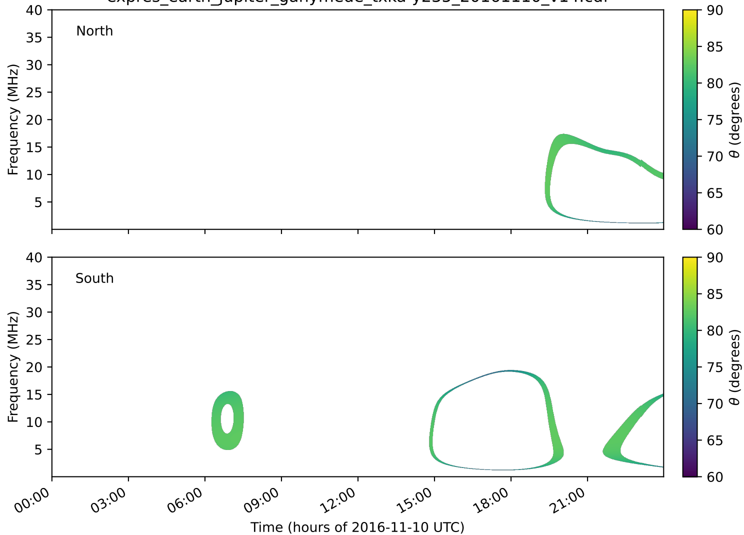
expres_earth_jupiter_ganymede_txka-y235_20161110_v14.cdf
