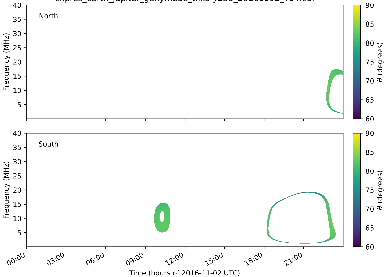
expres_earth_jupiter_ganymede_txka-y235_20161102_v14.cdf
