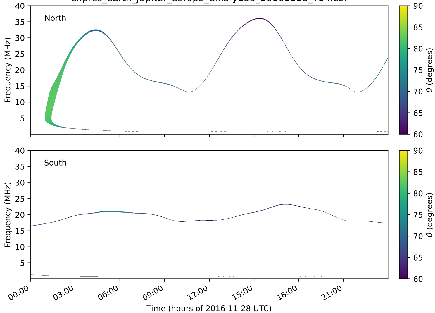
expres_earth_jupiter_europa_txka-y235_20161128_v14.cdf
