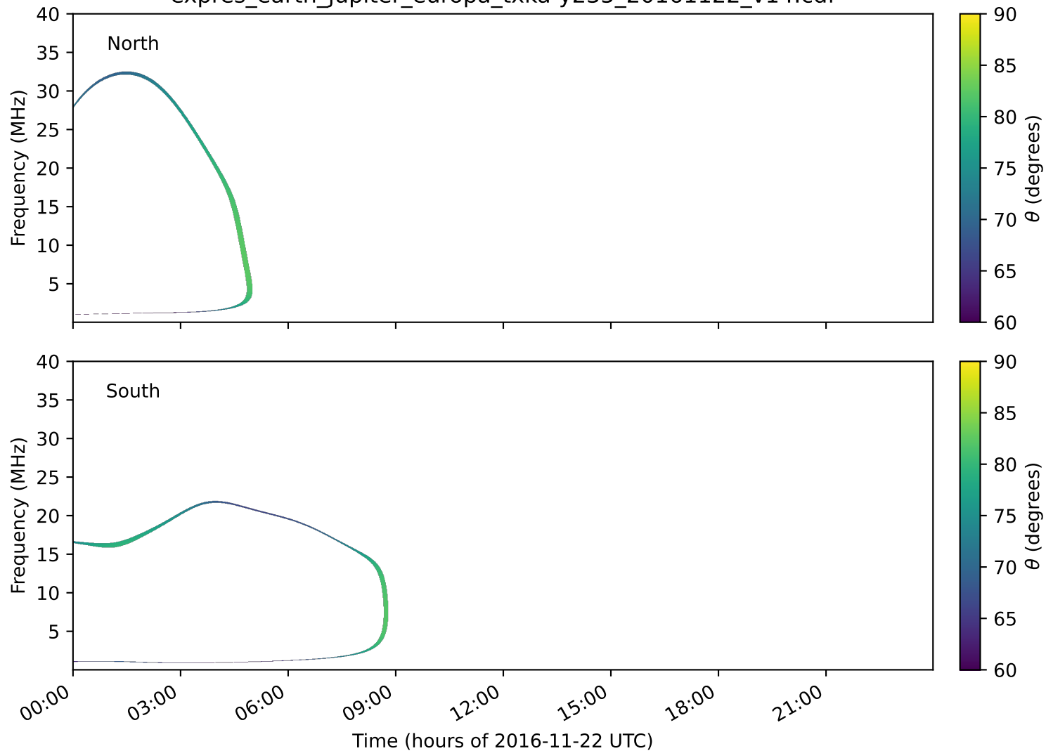
expres_earth_jupiter_europa_txka-y235_20161122_v14.cdf
