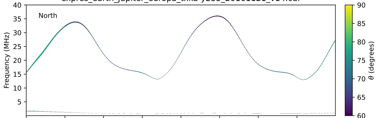
expres_earth_jupiter_europa_txka-y235_20161121_v14.cdf
