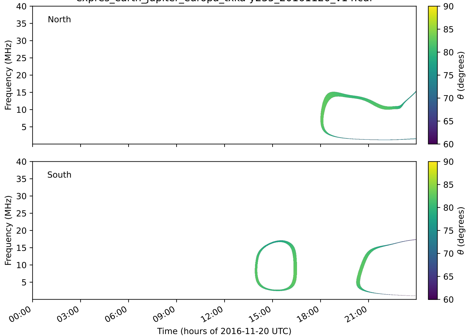
expres_earth_jupiter_europa_txka-y235_20161120_v14.cdf
