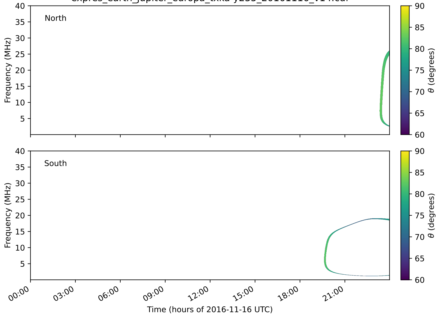
expres_earth_jupiter_europa_txka-y235_20161116_v14.cdf
