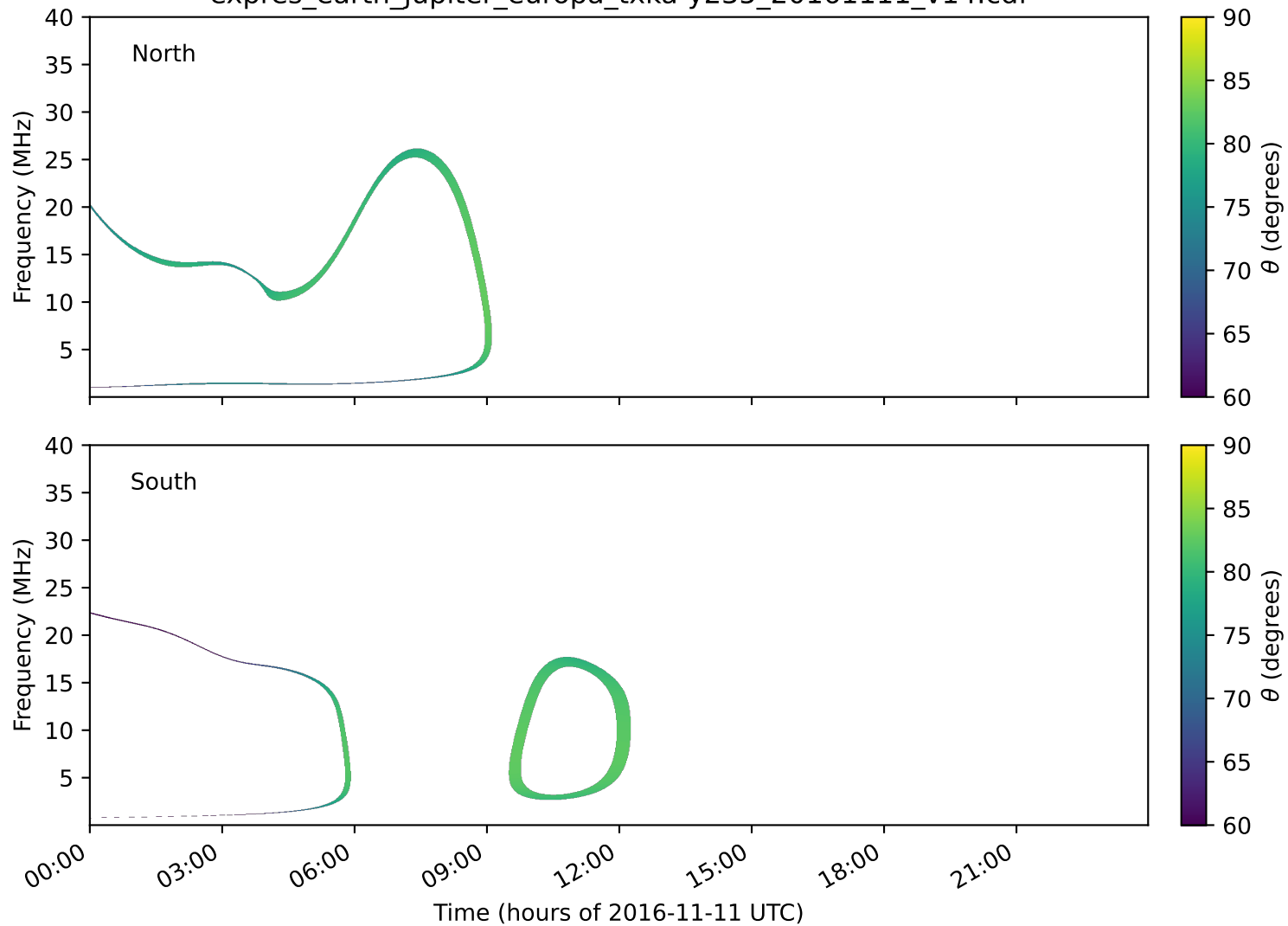
expres_earth_jupiter_europa_txka-y235_20161111_v14.cdf
