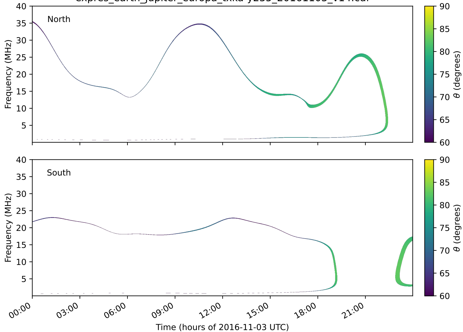
expres_earth_jupiter_europa_txka-y235_20161103_v14.cdf
