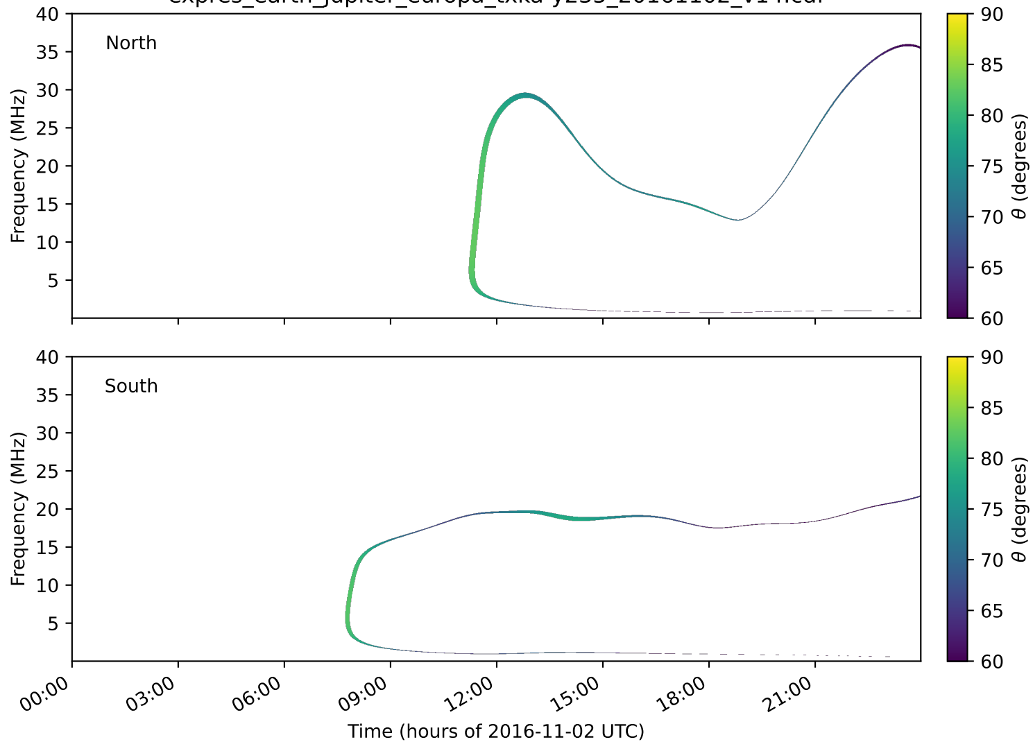
expres_earth_jupiter_europa_txka-y235_20161102_v14.cdf
