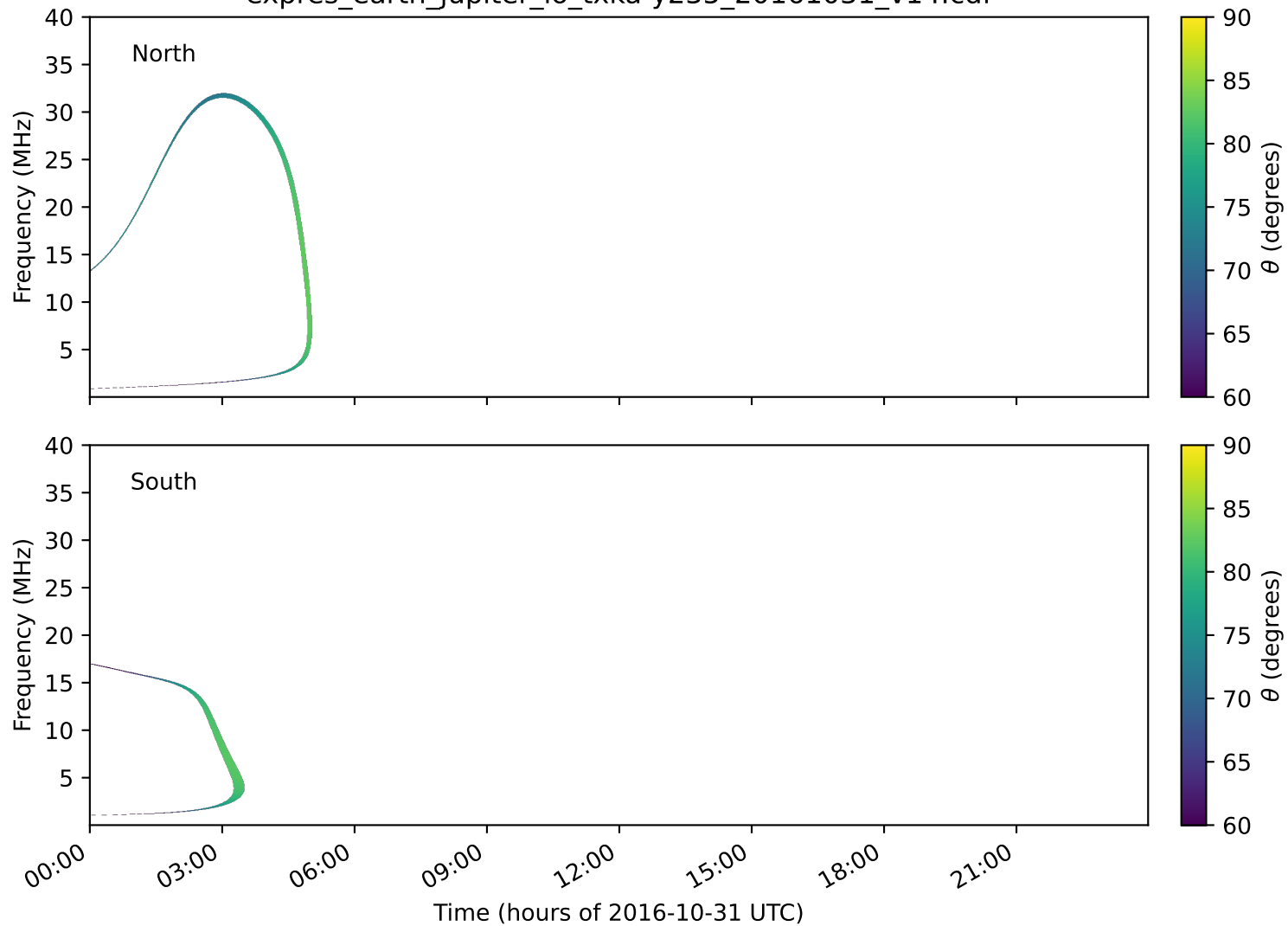
expres_earth_jupiter_io_txka-y235_20161031_v14.cdf
