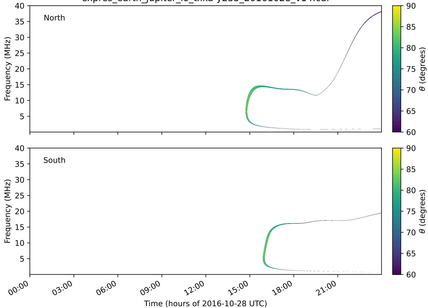
expres_earth_jupiter_io_txka-y235_20161028_v14.cdf
