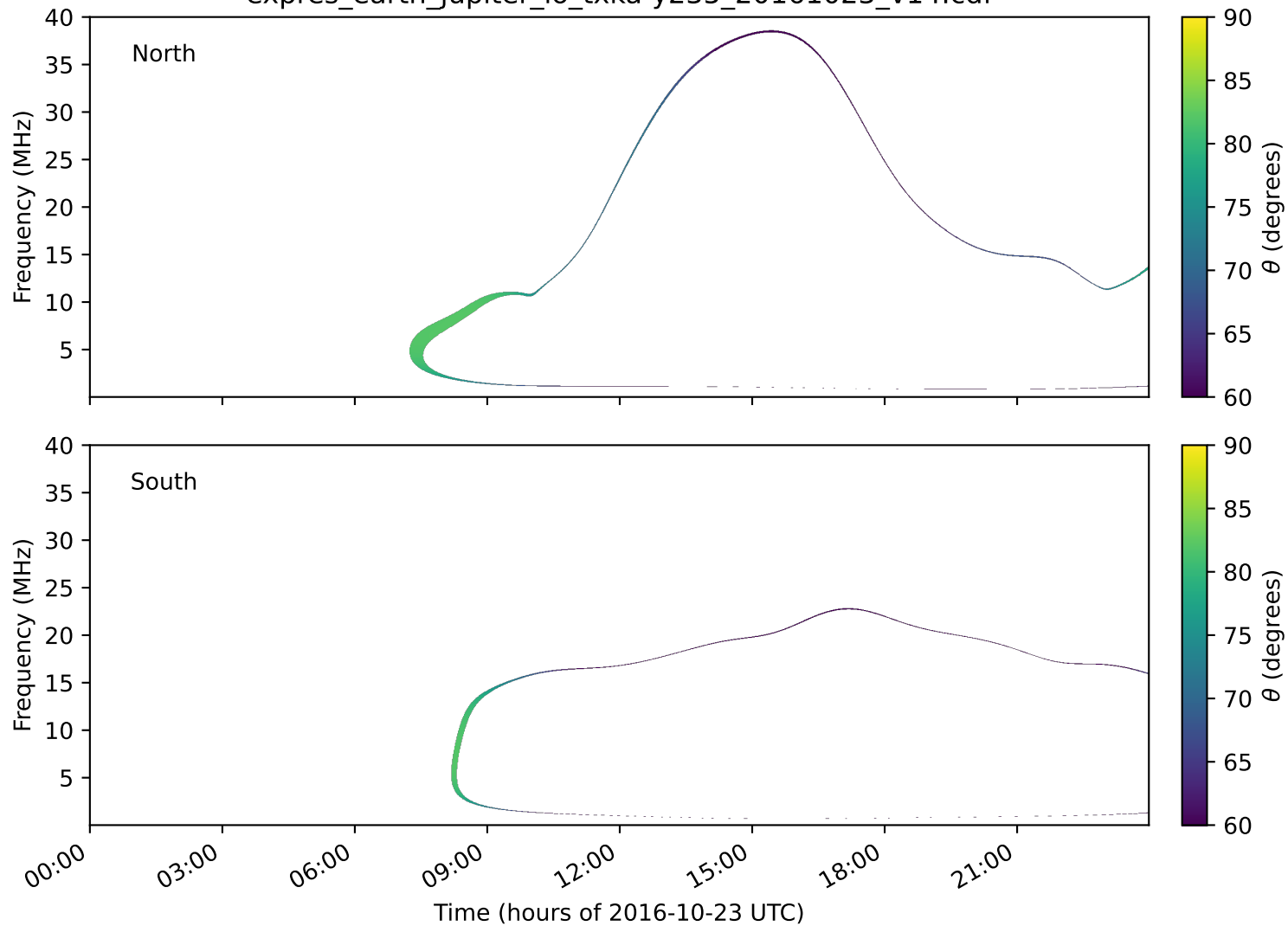
expres_earth_jupiter_io_txka-y235_20161023_v14.cdf
