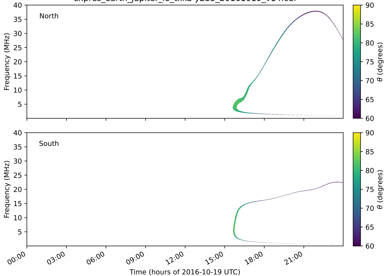
expres_earth_jupiter_io_txka-y235_20161019_v14.cdf
