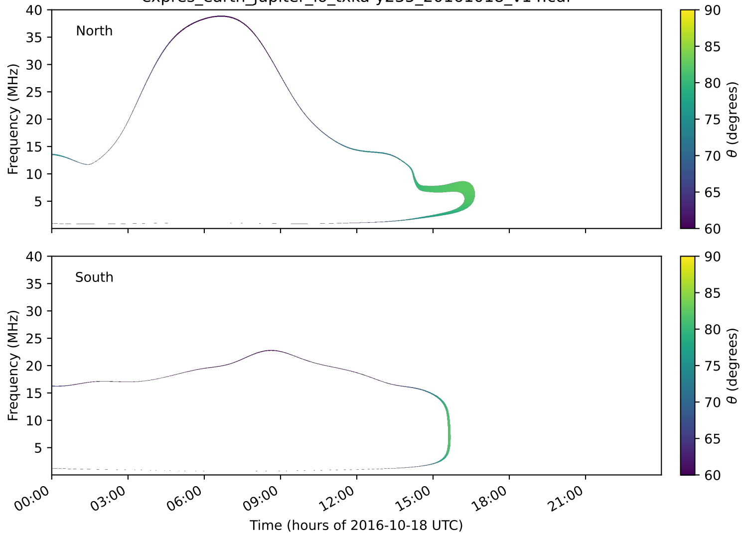
expres_earth_jupiter_io_txka-y235_20161018_v14.cdf
