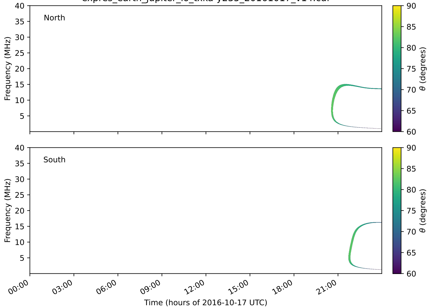
expres_earth_jupiter_io_txka-y235_20161017_v14.cdf
